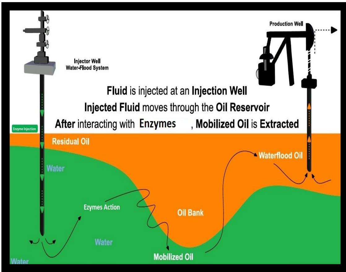
Figure 5 – Enzymes in Waterflooding process
