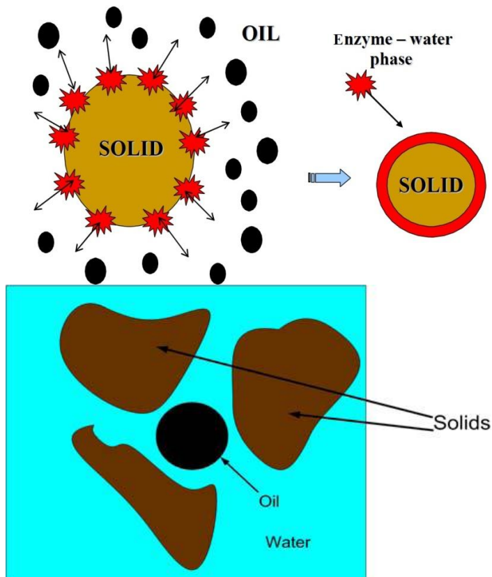
Figure 4 – EEOR in water wet systems
